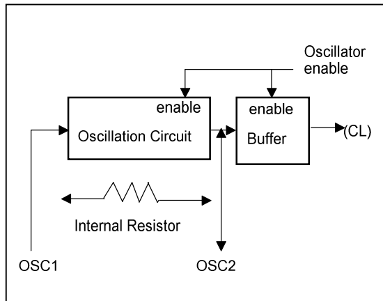
Figure 4 : Oscillator Circuit
