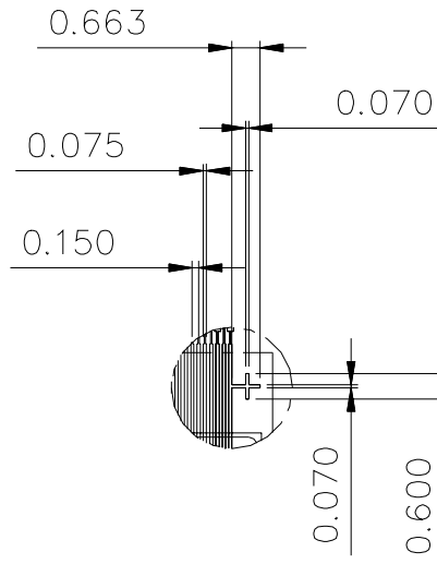
DETAIL B
