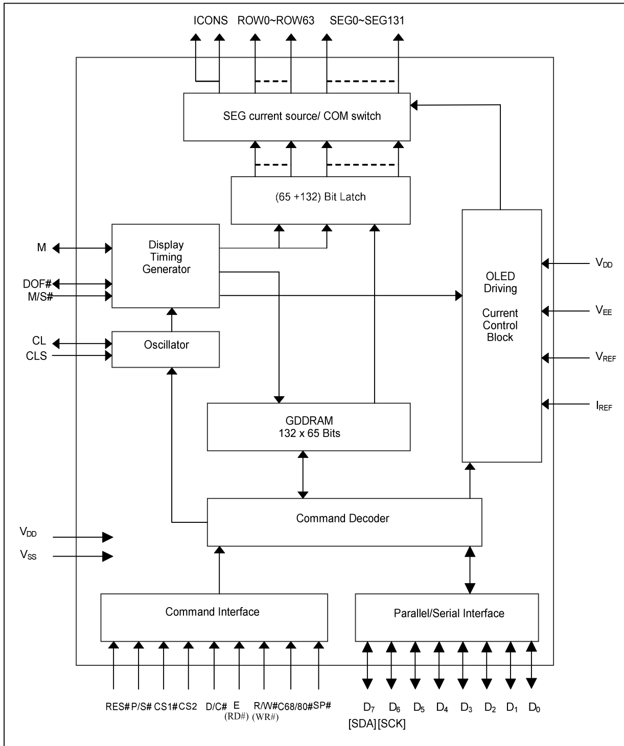
Figure 1 - Block Diagram
