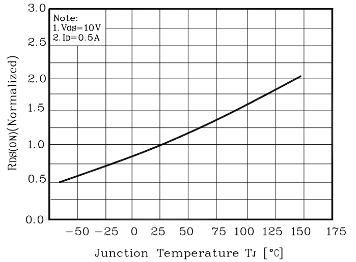
Fig. 8 R_{DS(on)} - T_J
