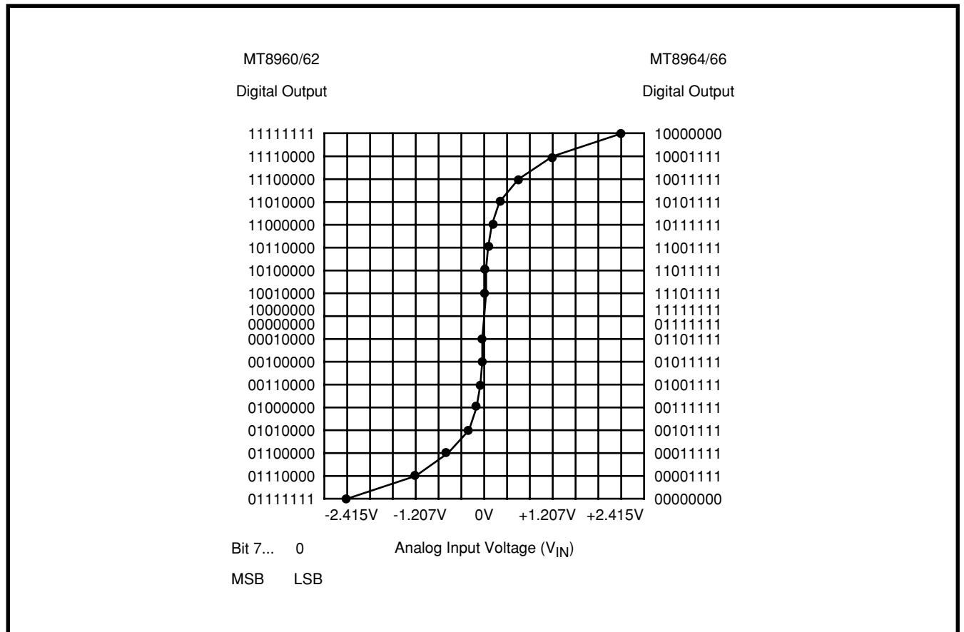
Figure 3 - \mu -Law Encoder Transfer Characteristic
