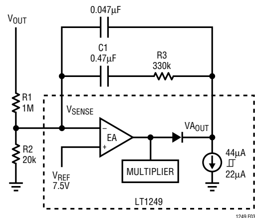
Figure 3. Overvoltage Protection
