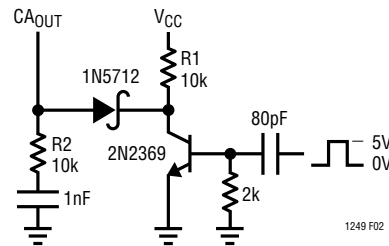
Figure 2. Synchronizing the LT1249
