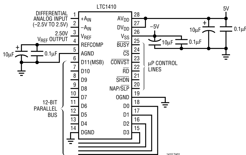
Complete 1.25MHz, 12-Bit Sampling A/D Converter
