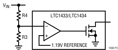
Figure 12. Low-Battery Comparator
