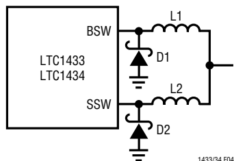
Figure 4. Using Two Inductors for Higher Low Current Efficiency
