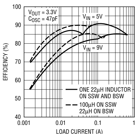
Figure 5. Efficiency Comparison Between Single Inductor and Dual Inductor
