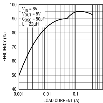
Figure 14. Design Example Circuit and its Efficiency Curve
