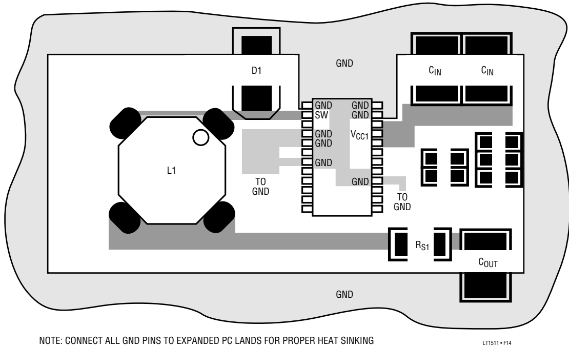
Figure 14. Critical Electrical and Thermal Path Layout
