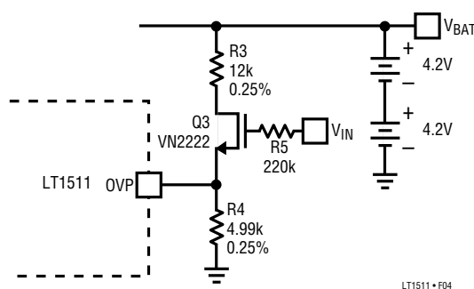
Figure 4. Disconnecting Voltage Divider
