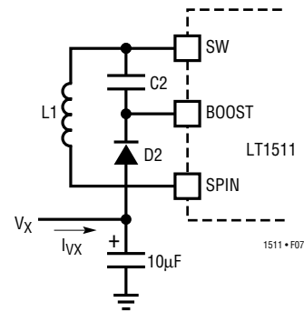
Figure 7. Lower V_{BOOST}
