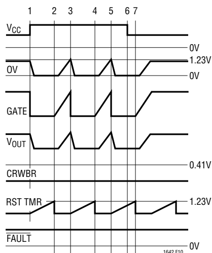
Figure 10. Overtiming (Low Side)
