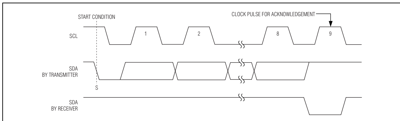
Figure 9. Acknowledge
