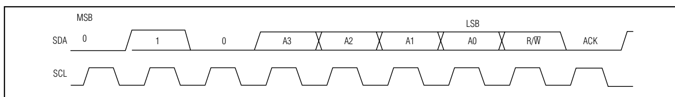
Figure 10. Slave Address
