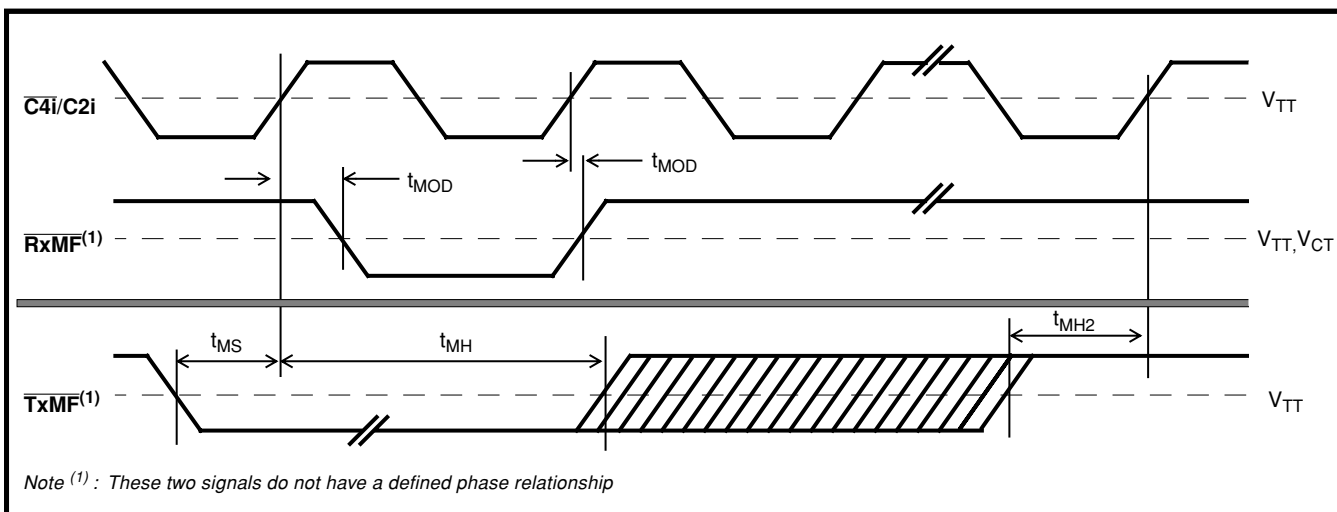
Figure 25 - Multiframe Timing Diagram ( \overline{C4i}/C2i = 2.048 MHz)
