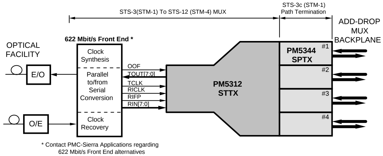
Figure 2 - 622 Mbit/s SONET/SDH Add-Drop Multiplexer Aggregate Interface
