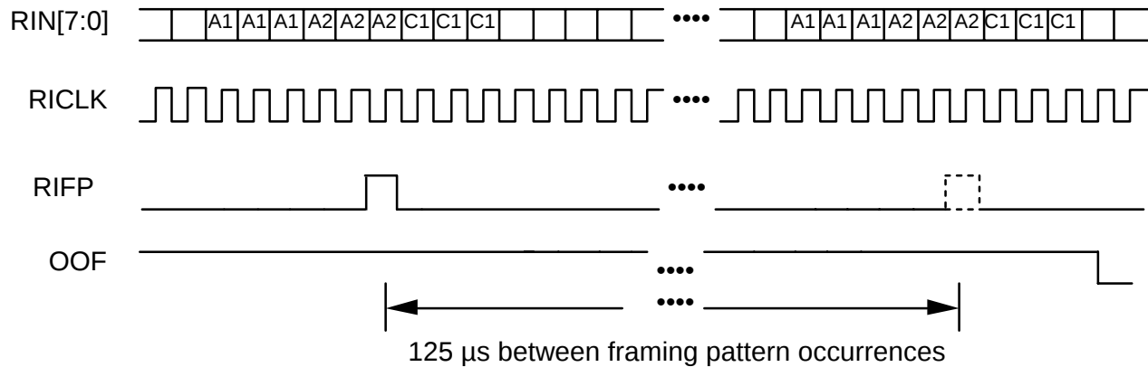
Figure 13 - In Frame Declaration
