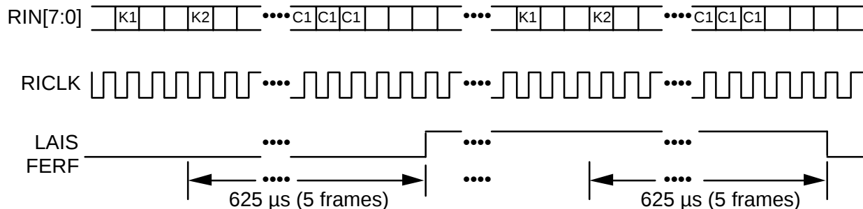
Figure 17 - Line AIS and Line FFERF Declaration/Removal
