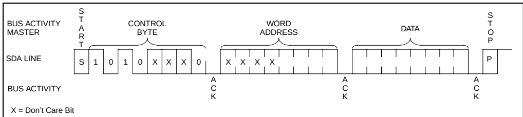
FIGURE 7-2: BYTE WRITE
