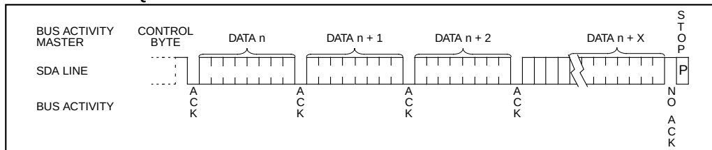
FIGURE 8-3: SEQUENTIAL READ
