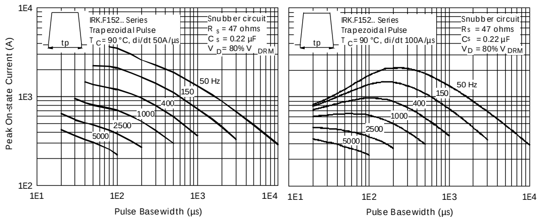
Fig. 12 - Frequency Characteristics
