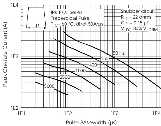
Fig. 12 - Frequency Characteristics
