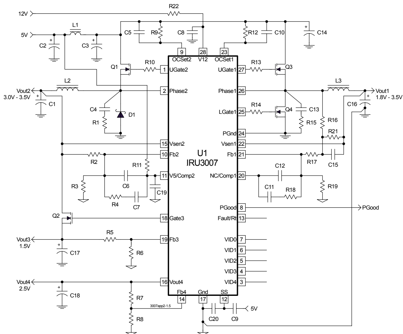
Figure 4 - Typical application of IRU3007 in a dual layout with HIP6019 for an on-board DC-DC converter providing power for the Vcore, GTL+, Clock supply as well as an on-board 3.3V I/O supply for the Deschutes and the next generation processor application.
