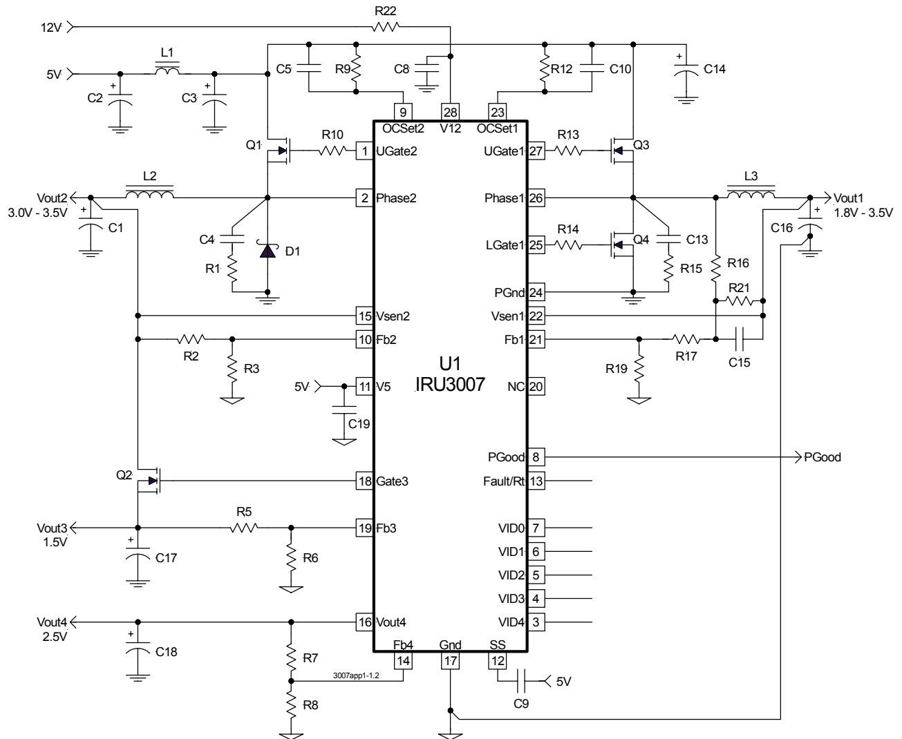
Figure 3 - Typical application of IRU3007 for an on-board DC-DC converter providing power for the Vcore, GTL+, Clock supply as well as an on-board 3.3V I/O supply for the Deschutes and the next generation processor applications.
