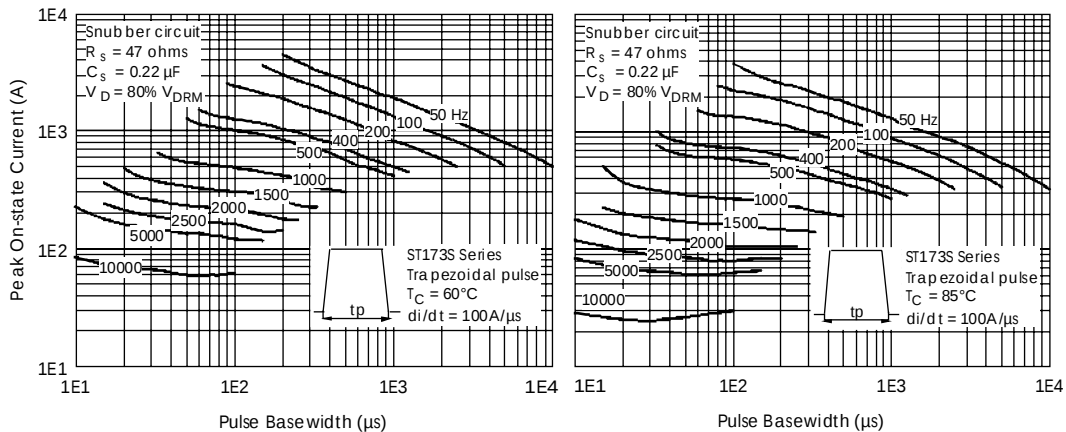
Fig. 13 - Frequency Characteristics
