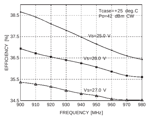
Efficiency vs Frequency
