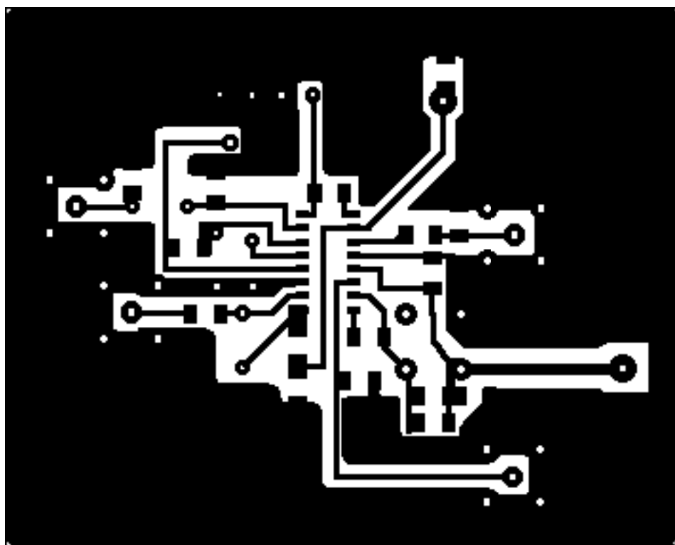
Fig. 18 Track side of demonstration board. Scale = 2:1.
