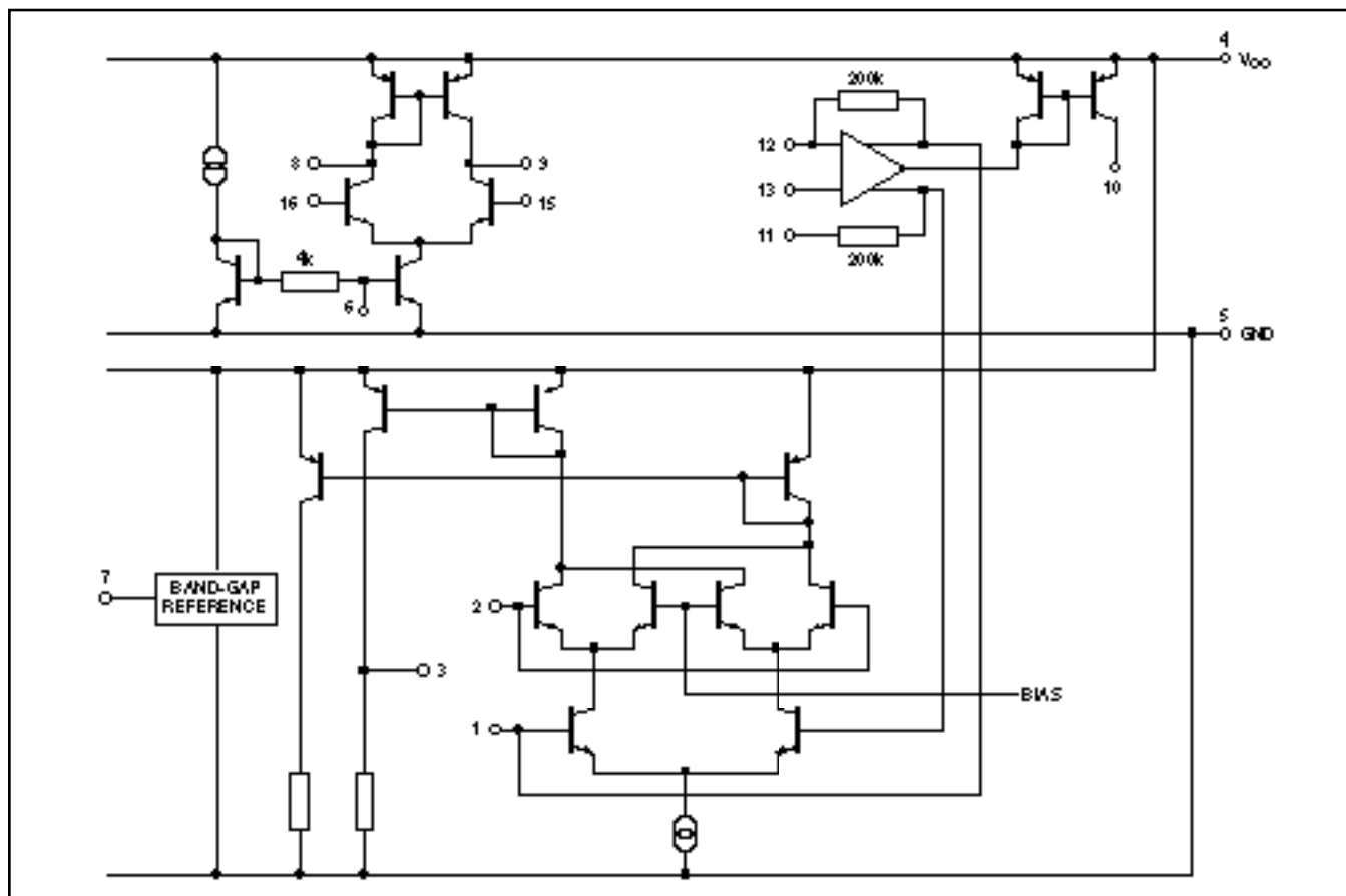
Fig. 3 Internal schematic
