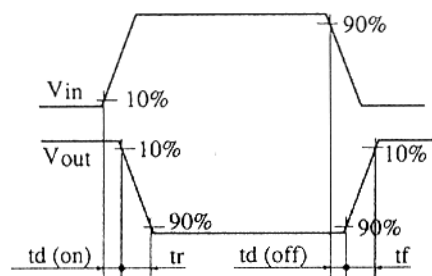
SWITCHING TIME TEST WAVEFORMS
