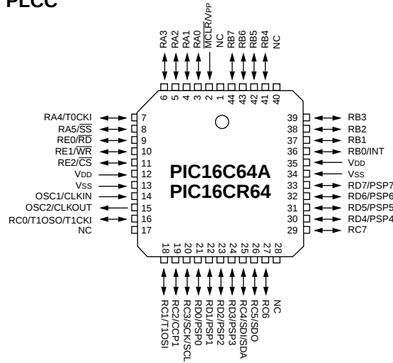
PLCC
