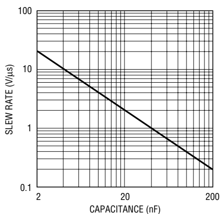
Figure 4. Slew Rate vs Capacitance
