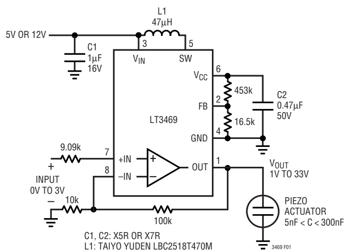
Figure 1. Differential Input Piezo Microactuator Driver
