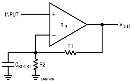
Figure 6. Boosting the Bandwidth of the g_m Amplifier with Capacitance On the Inverting Input
