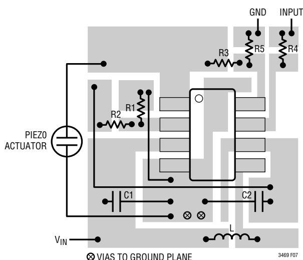
Figure 7. Recommended Component Placement
