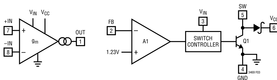
Figure 3. LT3469 Block Diagram
