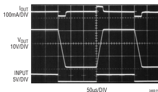
Figure 2. Response Driving a 33nF Load
