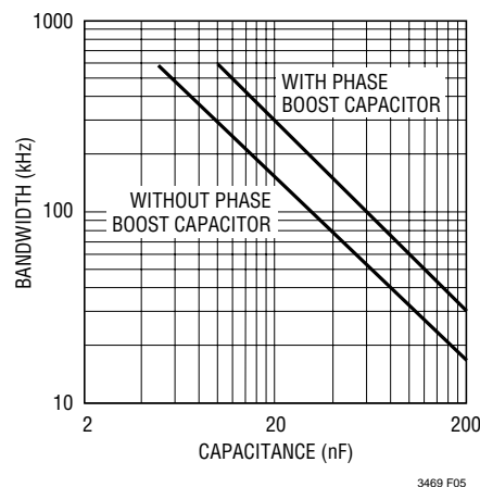
Figure 5. Closed Loop -3 dB Bandwidth vs Capacitance in a Gain of 10 Configuration
