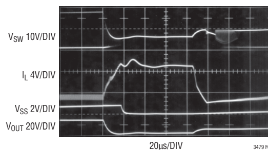
Figure 9. Output Overload with Inrush Current Protection Enabled
