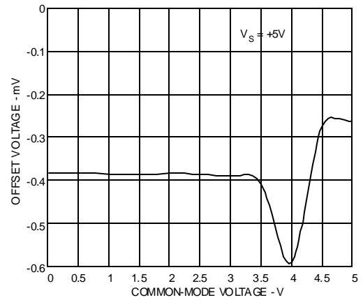
Figure 35. V_{OS} vs Common-Mode Voltage
