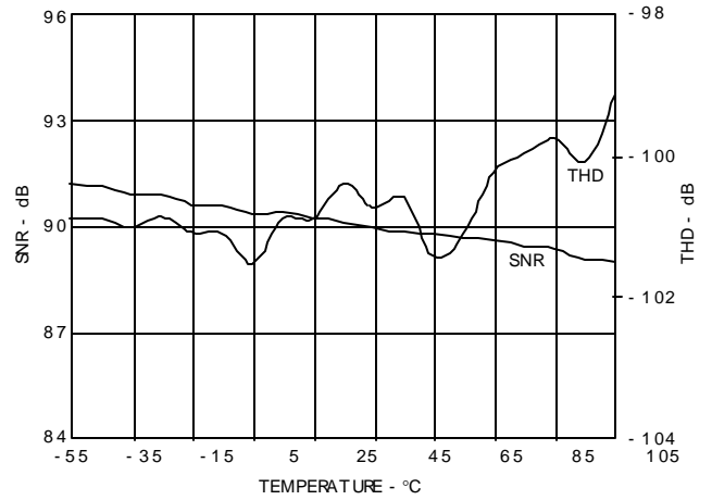
Figure 13. SNR, THD vs Temperature
