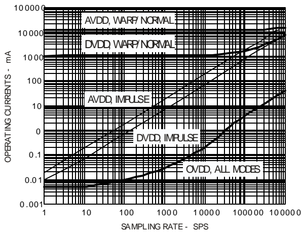
Figure 17. Operating Currents vs Sample rate
