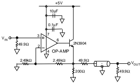
Figure 104. Low Distortion Line Driver for Single Supply Ground Referenced Signals
