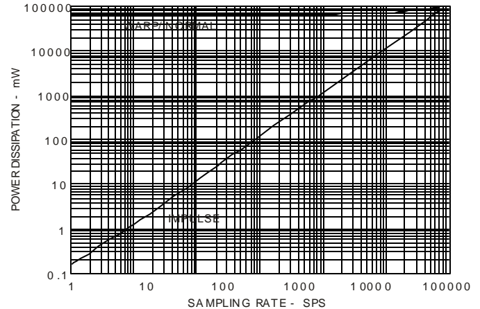
Figure 74. Power Dissipation vs. Sample Rate
