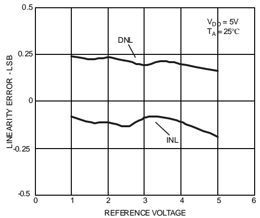
Figure 24. Linearity Error vs Reference Voltage
