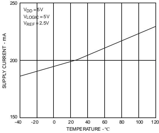
Figure 26. Supply Current vs Temperature
