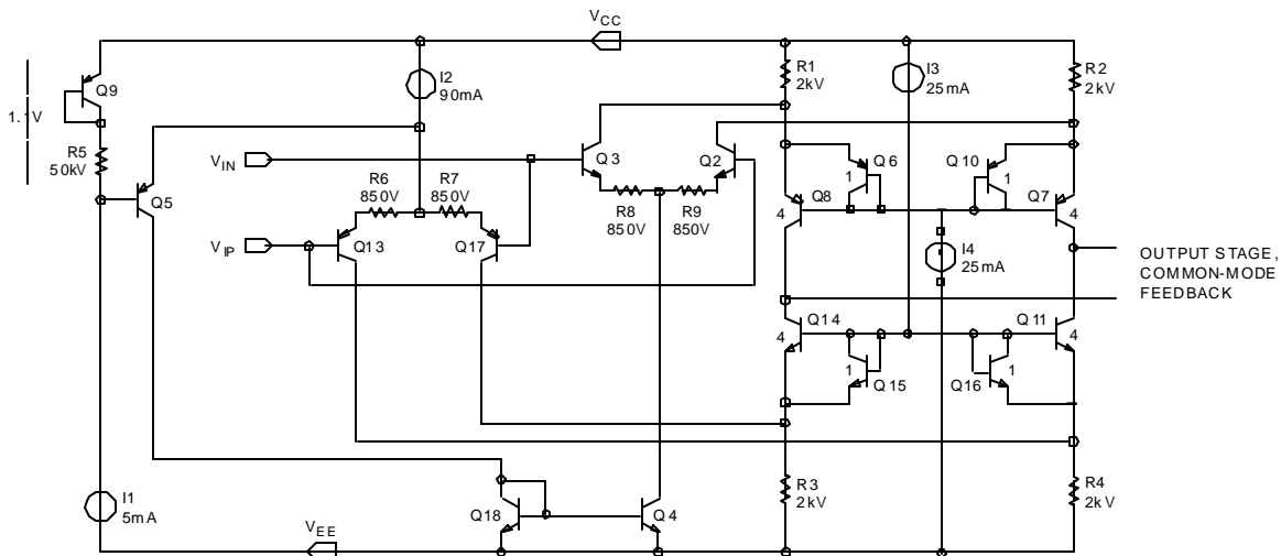
Figure 100. Simplified Schematic of Input Stage
