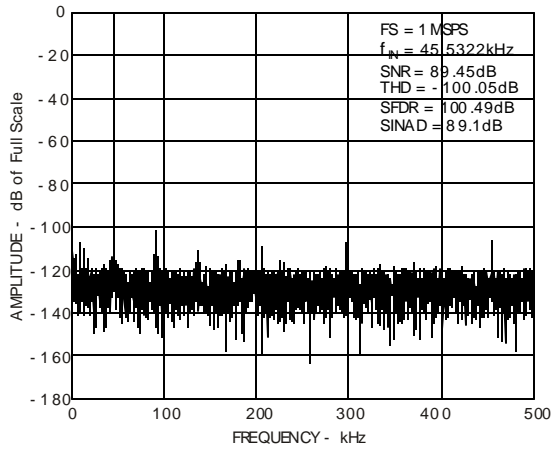
Figure 10. FFT Plot
