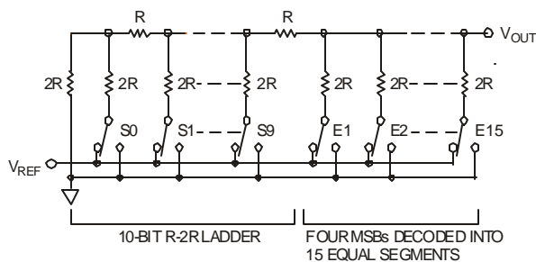
Figure 92. DAC Architecture
