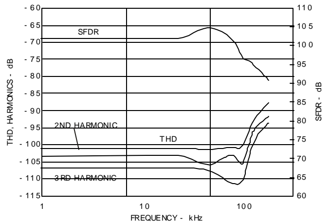
Figure 14. THD, Harmonics, and SFDR vs Frequency
