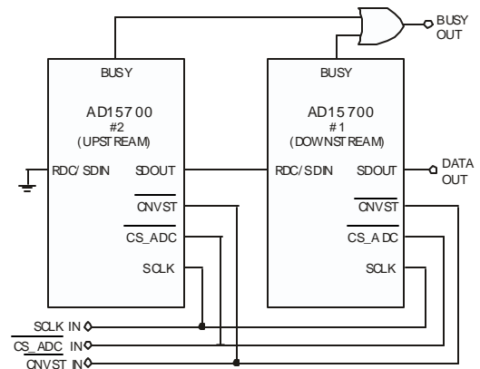
Figure 84. Two AD15700s in a Daisy-Chain Configuration
