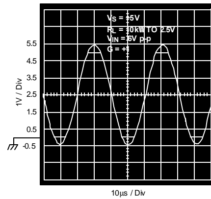
Figure 59. Output Voltage
