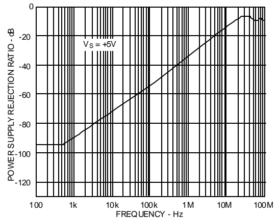
Figure 58. PSRR vs Frequency
