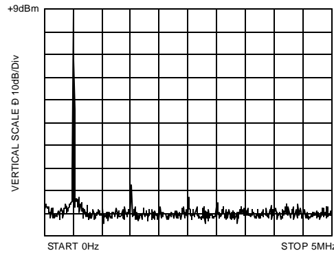
Figure 106. THD of Low Distortion Line Driver at 500 kHz
