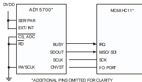
Figure 86. Interfacing the AD15700 to SPI Interface
