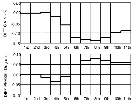
Figure 47. Differential Gain and Phase @ V_S = \pm 5V ; R_L = 1k\Omega
