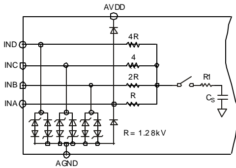
Figure 70. Simplified Analog Input
