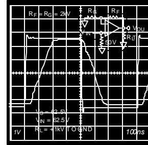
Figure 102. Overdrive Recovery
