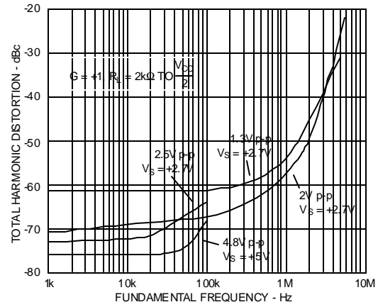
Figure 53. Total Harmonic Distortion vs Frequency; G=+1
