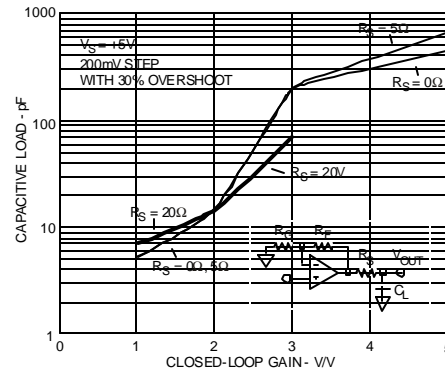
Figure 103. Capacitive Load Drive vs. Closed-Loop Gain
