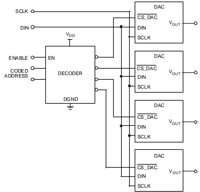
Figure 99. Addressing Multiple DACs
