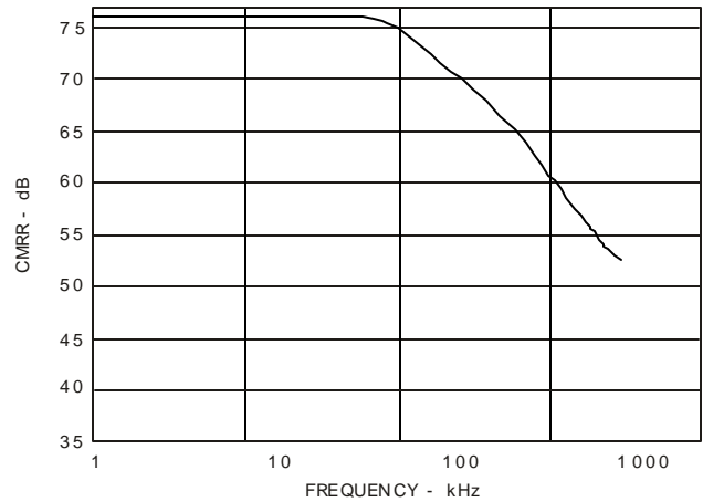
Figure 71. Analog Input CMRR vs. Frequency
