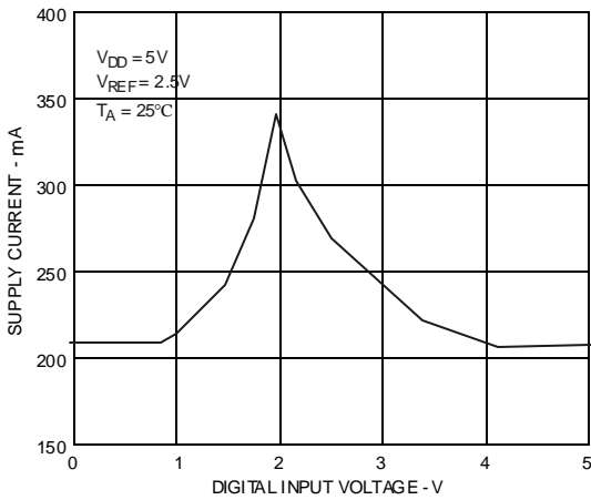
Figure 27. Supply Current vs Digital Input Voltage
