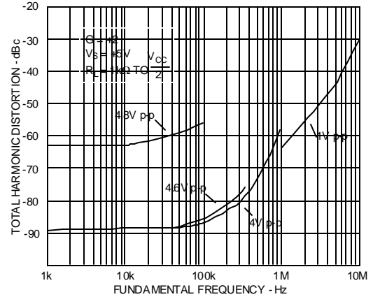
Figure 54. Total Harmonic Distortion vs Frequency; G=+2
