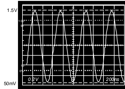
Figure 107. Output Signal Swing of Low Distortion Line Driver at 2 MHz
