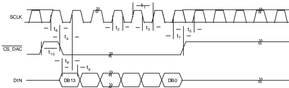
Figure 3. Timing Diagram
