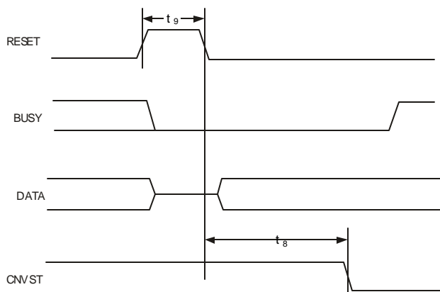
Figure 76. RESET Timing
