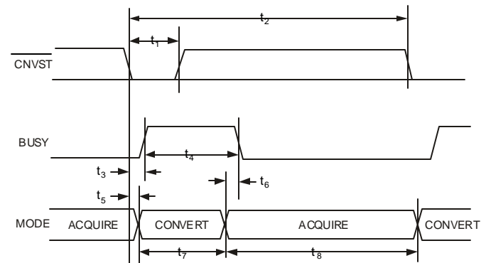
Figure 75. Basic Conversion Timing
