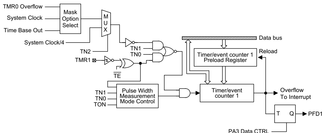
Timer/event counter 1
