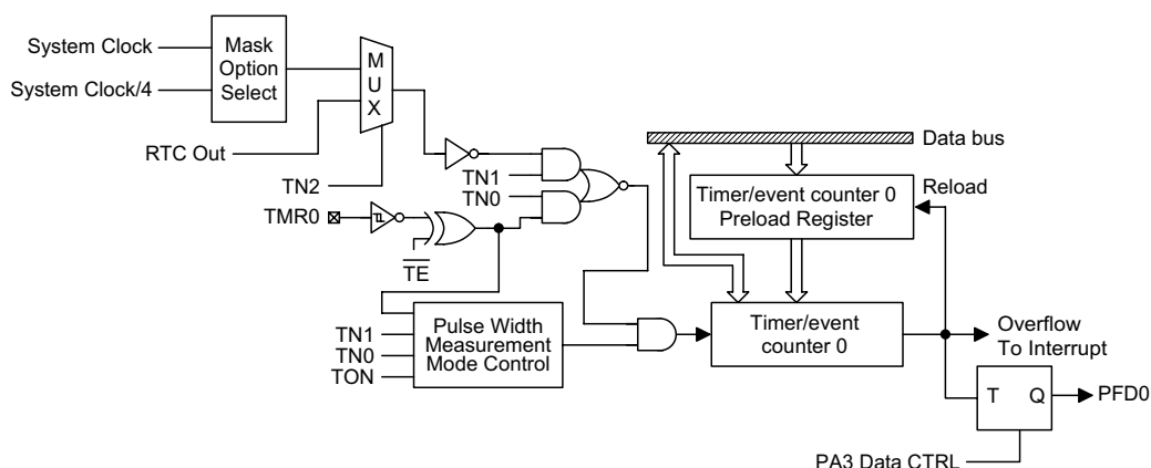
Timer/event counter 0
