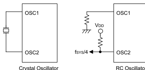
System oscillator
