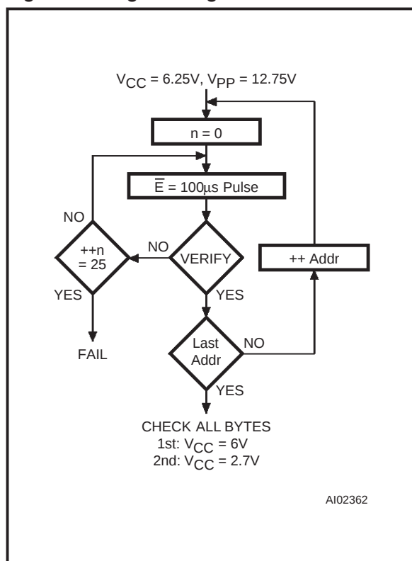
Figure 8. Programming Flowchart
