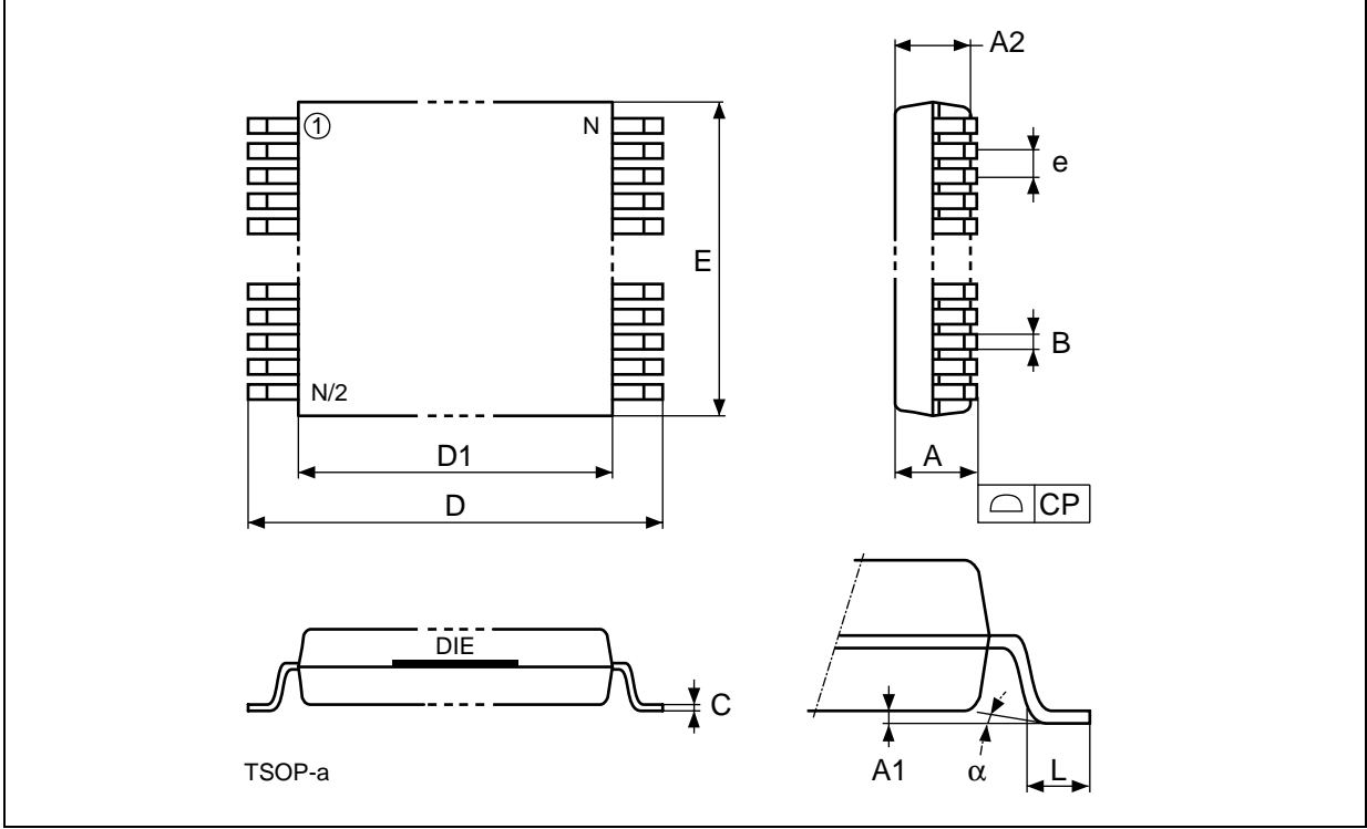
Figure 11. TSOP32 - 32 lead Plastic Thin Small Outline, 8 x 20mm, Package Outline
