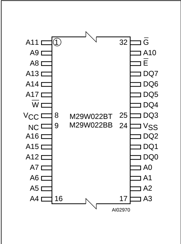
Figure 2A. TSOP Connections
