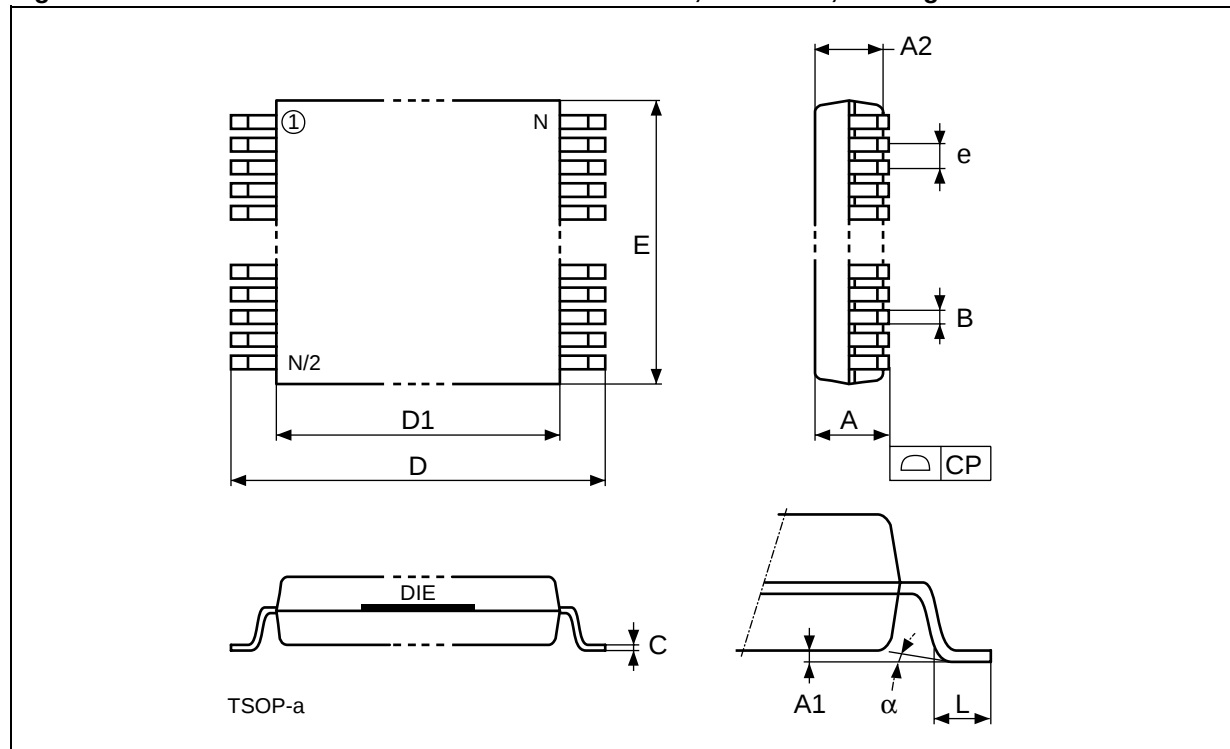
Figure 10. TSOP32 - 32 lead Plastic Thin Small Outline, 8 x 14mm, Package Outline
