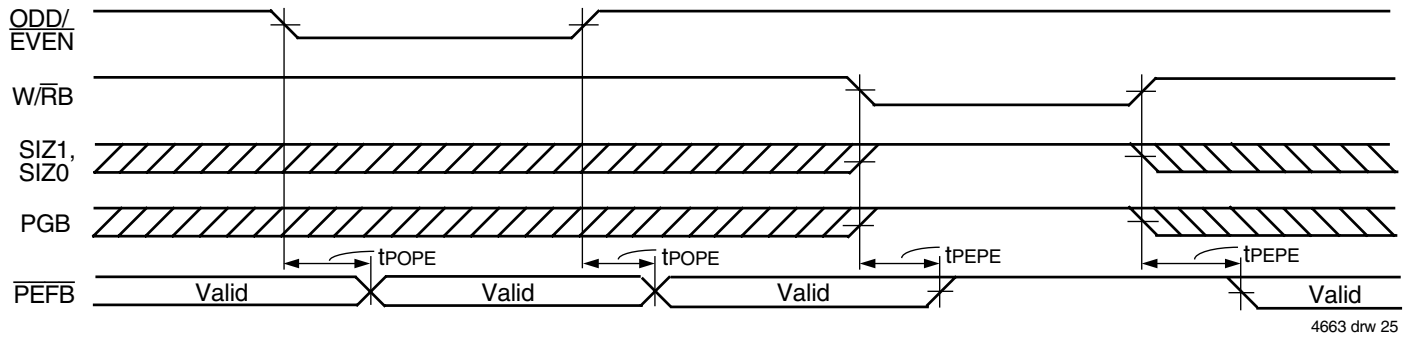
Figure 25. ODD/ \overline{\text{EVEN}} , \text{W}/\overline{\text{RB}} , SIZ1, SIZ0, and PGB to \overline{\text{PEFB}} Timing
