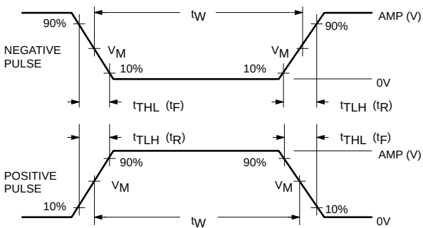
V_M = 1.5V Input Pulse Definition
