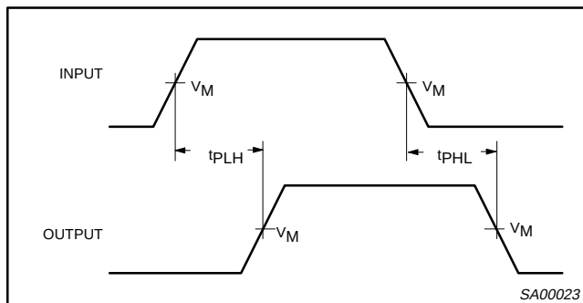
Waveform 4. Propagation Delay For Non-Inverting Output
