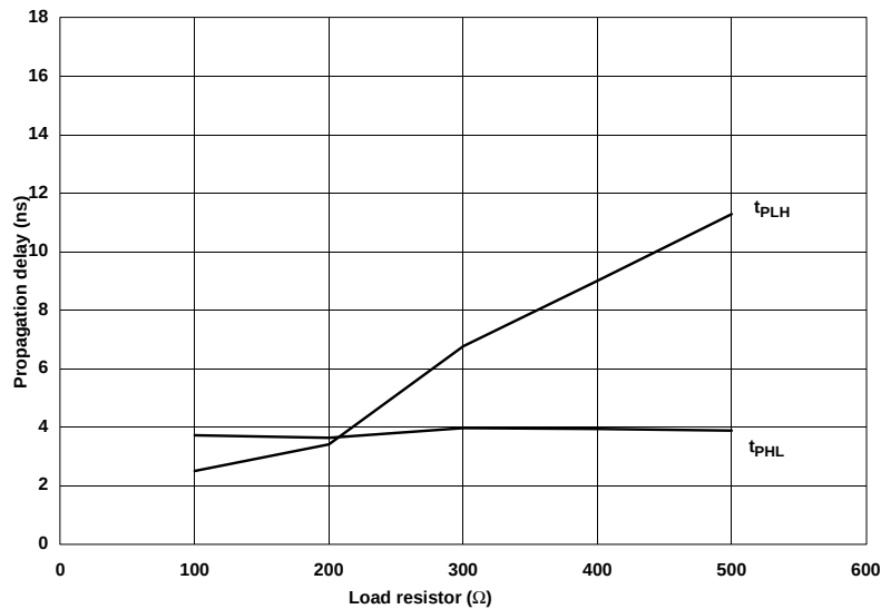
TYPICAL PROPAGATION DELAYS VERSUS LOAD FOR OPEN COLLECTOR OUTPUTS
