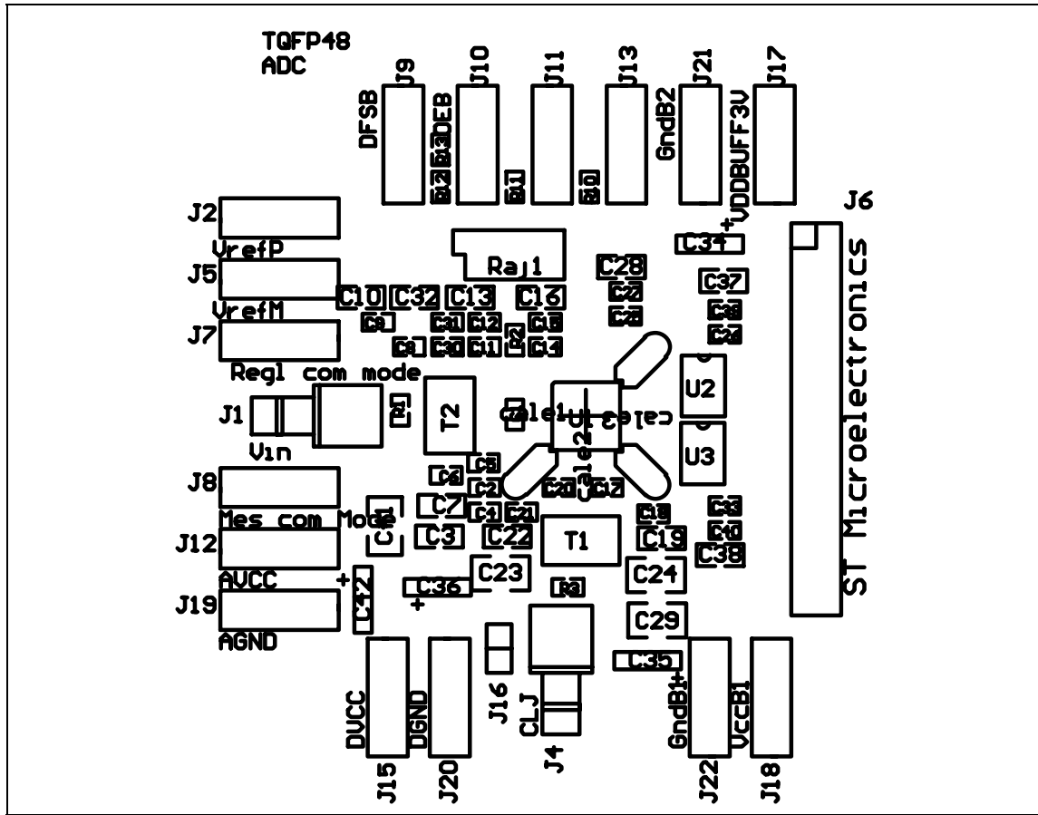
Figure 13 : Printed circuit of evaluation board.
