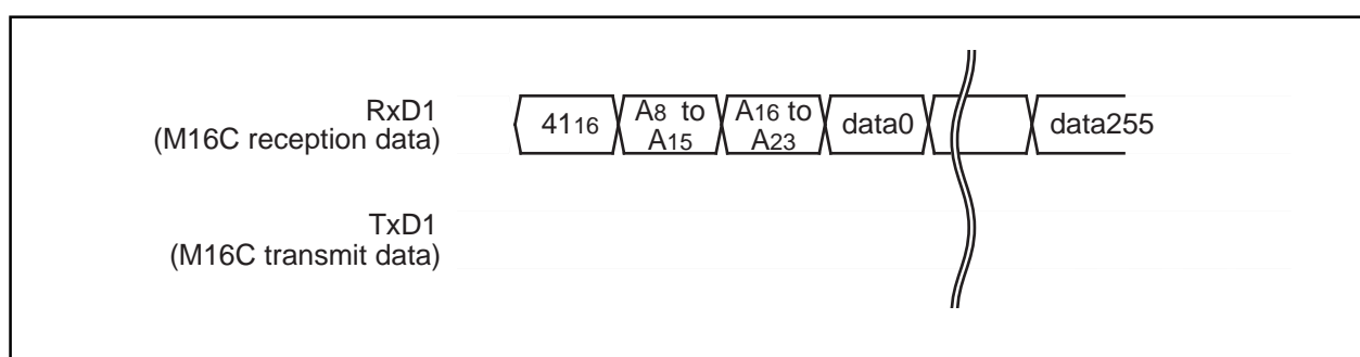
Figure 1.32.25. Timing for the page program
