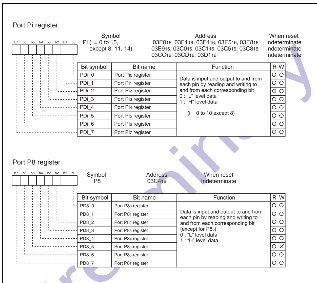
Figure 1.26.6. Port register (1)
