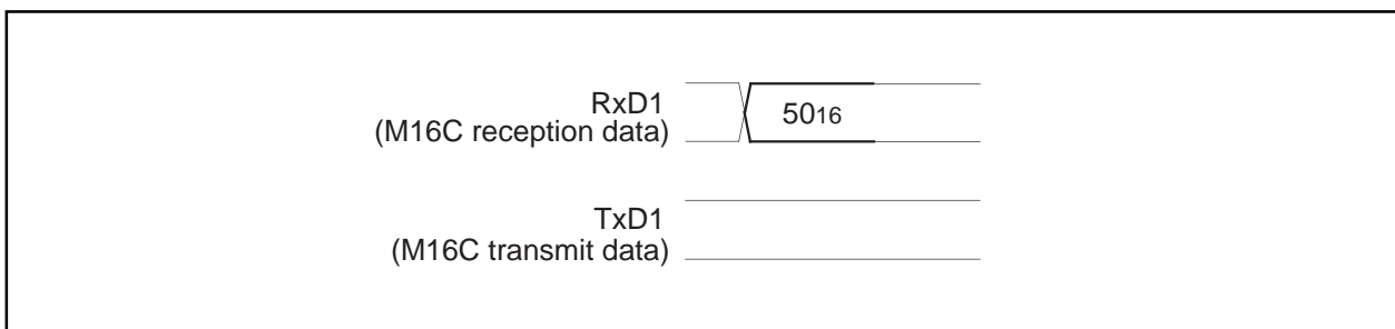
Figure 1.32.24. Timing for clearing the status register
