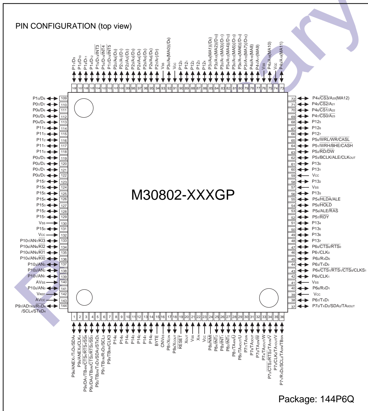
Figure 1.1.1. Pin configuration (top view)
