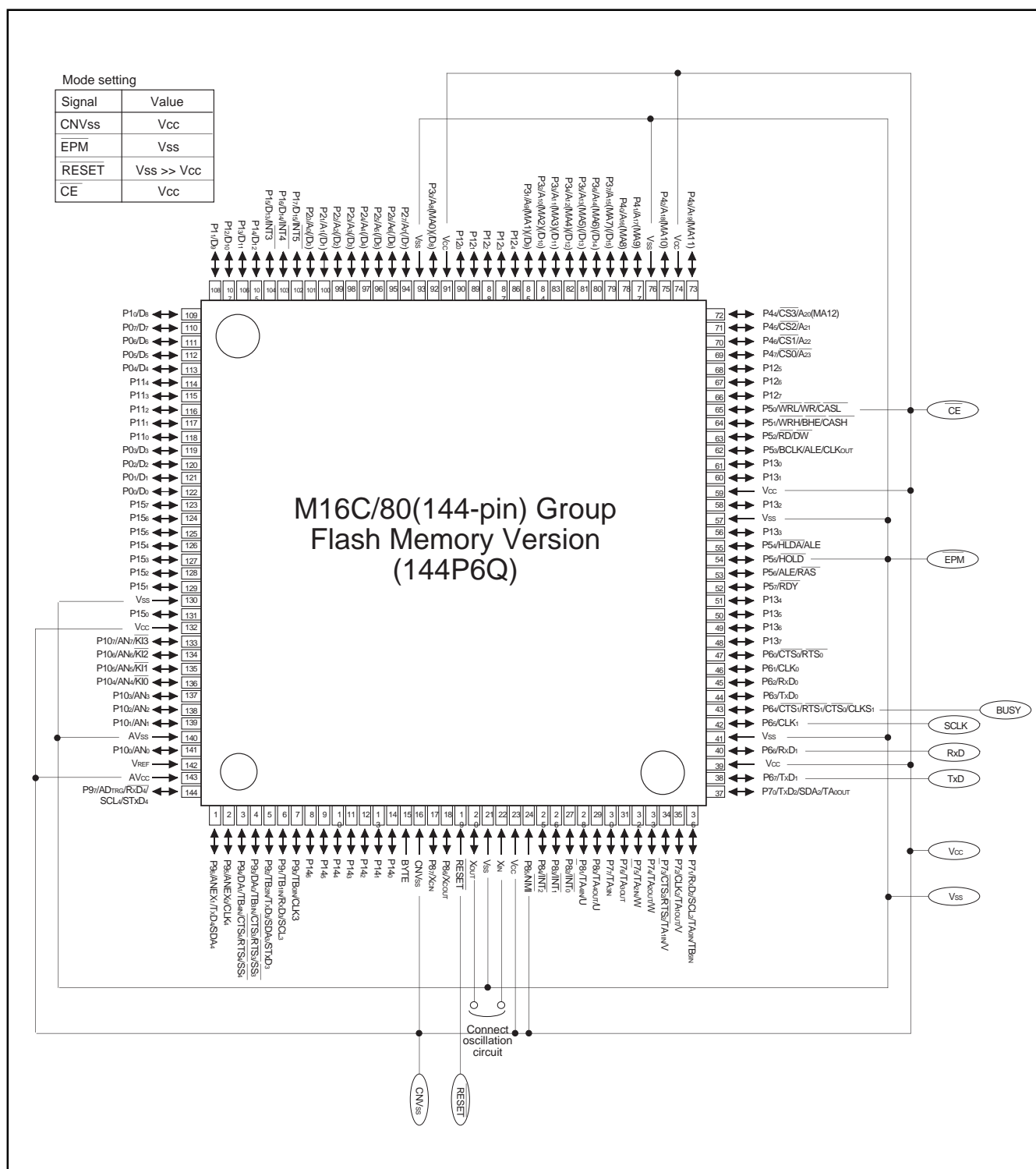
Figure 1.32.1. Pin connections for serial I/O mode
