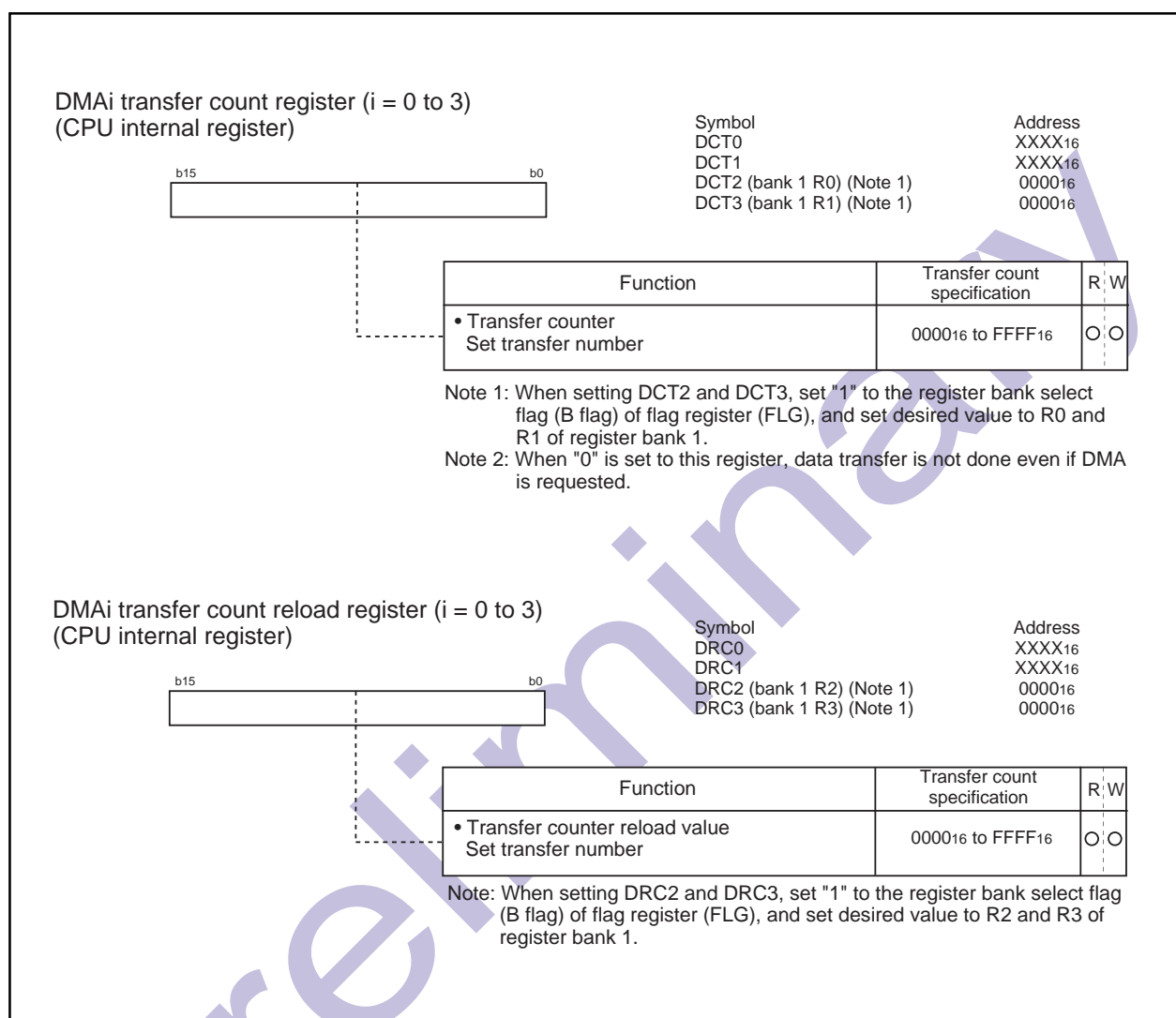
Figure 1.11.4. DMAC register (3)
