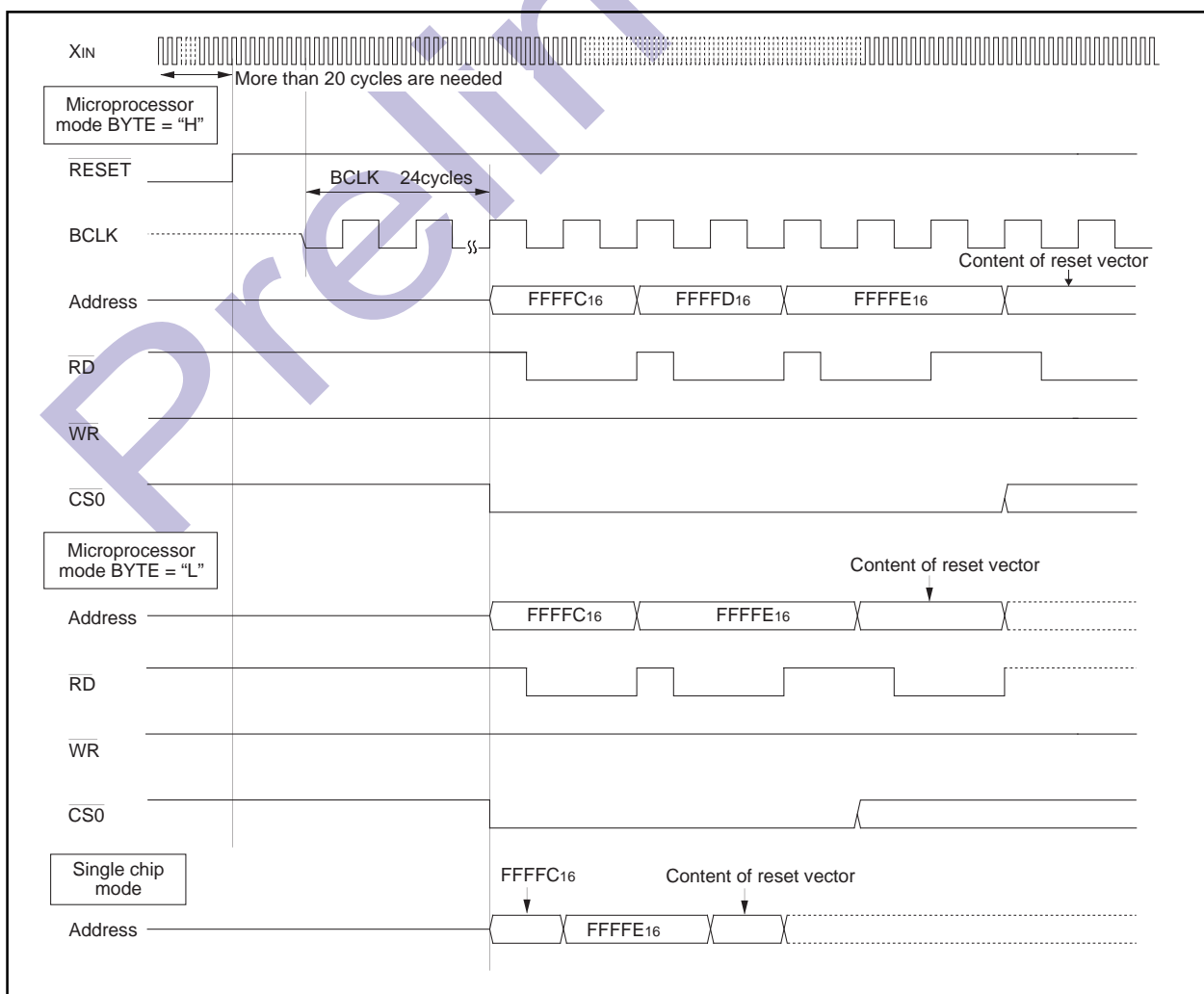
Figure 1.4.2. Reset sequence
