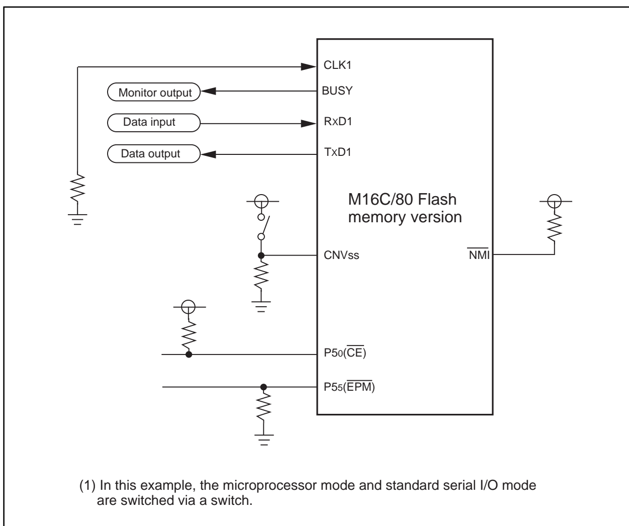
Figure 1.32.43. Example circuit application for the standard serial I/O mode 2
