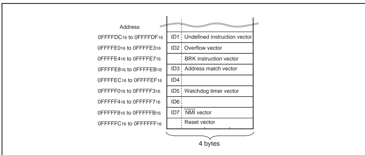
Figure 1.32.16. ID code storage addresses
