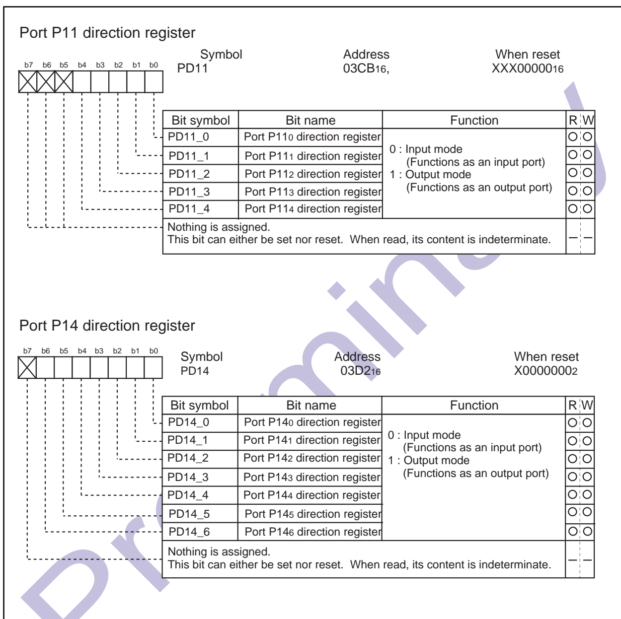
Figure 1.26.5. Direction register (2)
