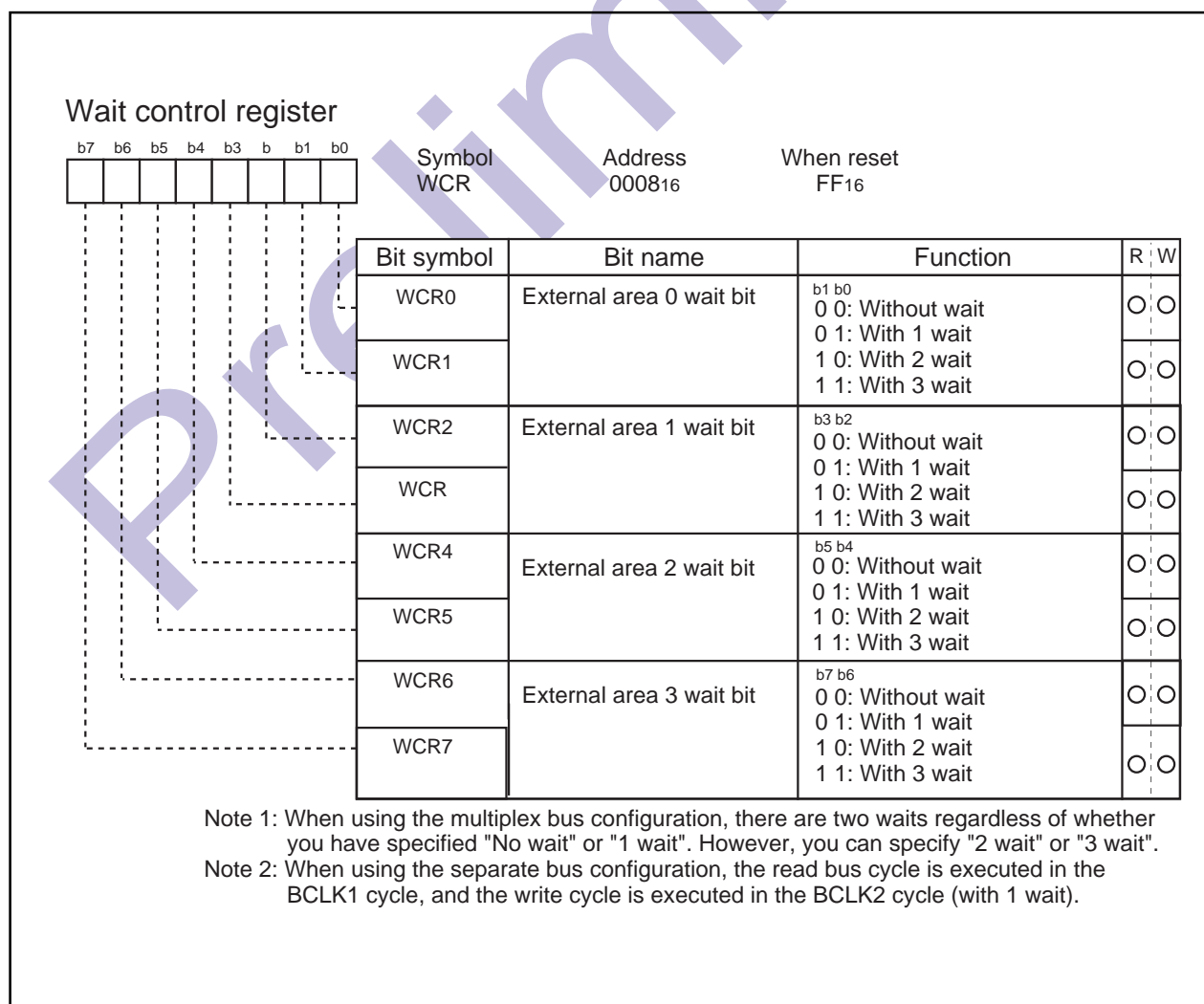
Figure 1.7.5. Wait control register
