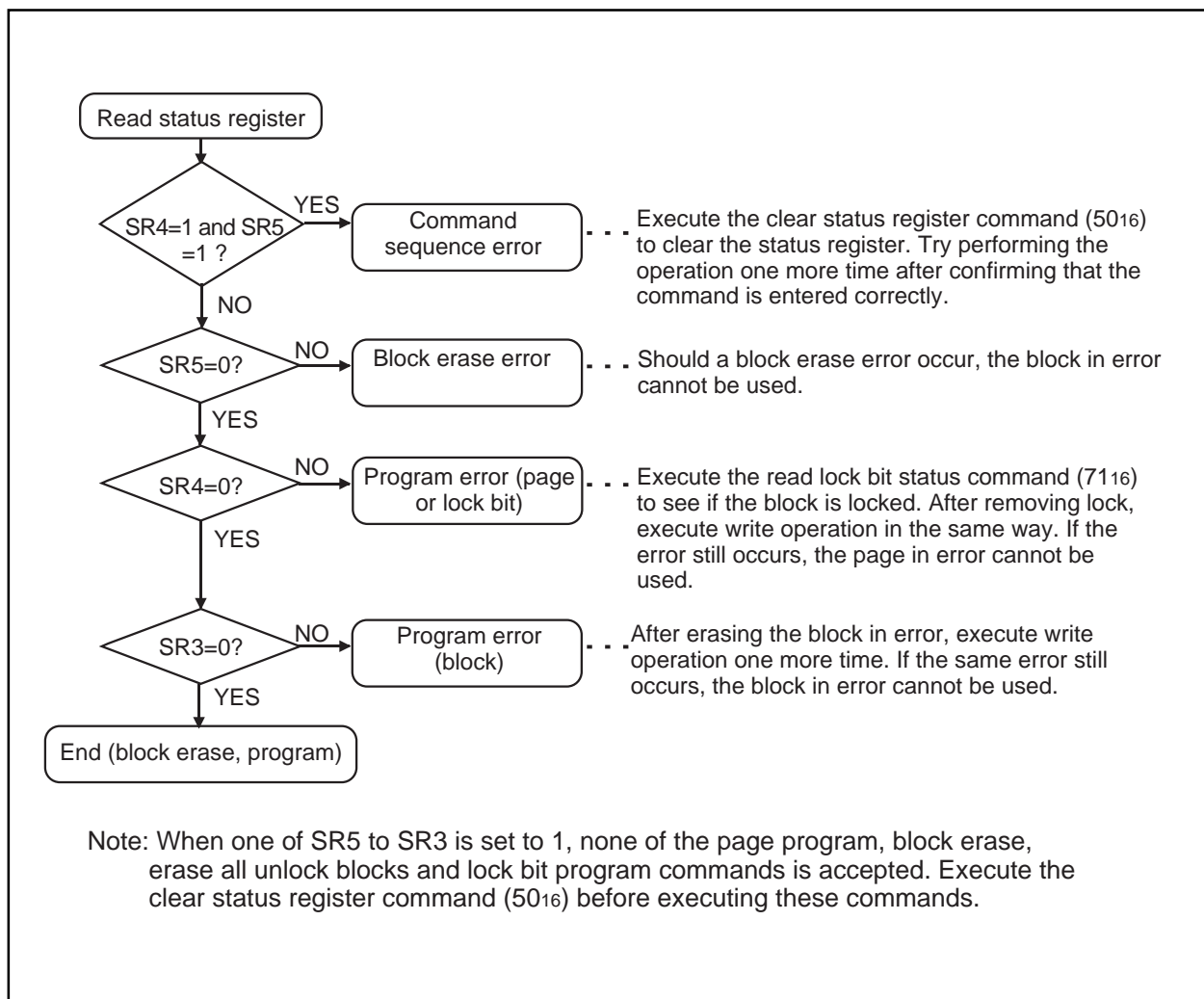
Figure 1.32.19. Full status check flowchart and remedial procedure for errors
