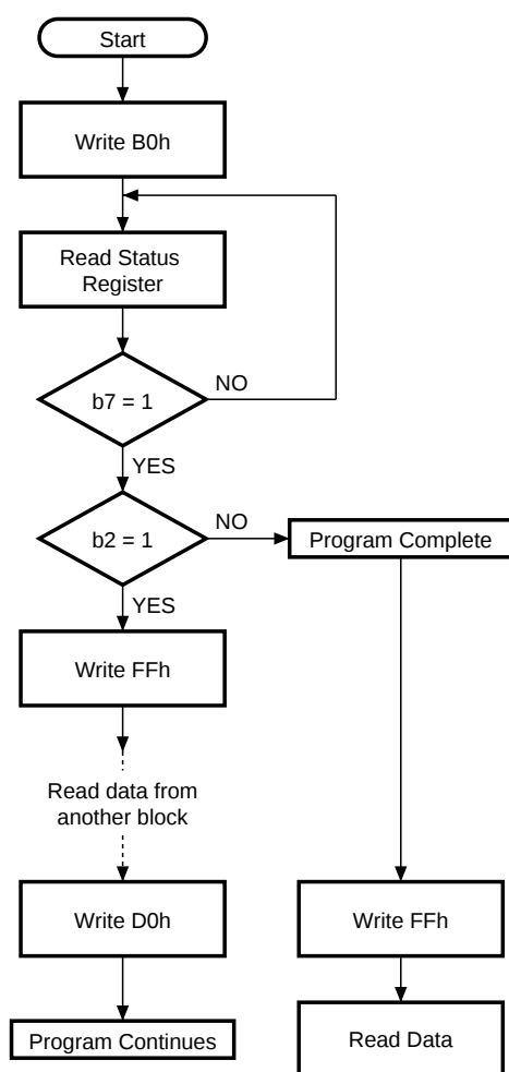
Figure 17. Program Suspend &amp; Resume Flowchart and Pseudo Code
