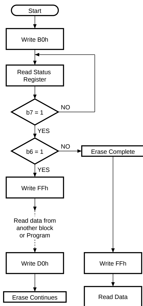
Figure 19. Erase Suspend &amp; Resume Flowchart and Pseudo Code
