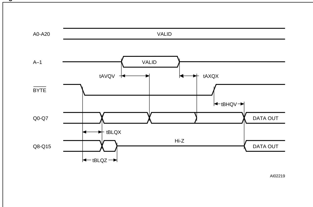
Figure 8. \overline{\text{BYTE}} Transition AC Waveforms
