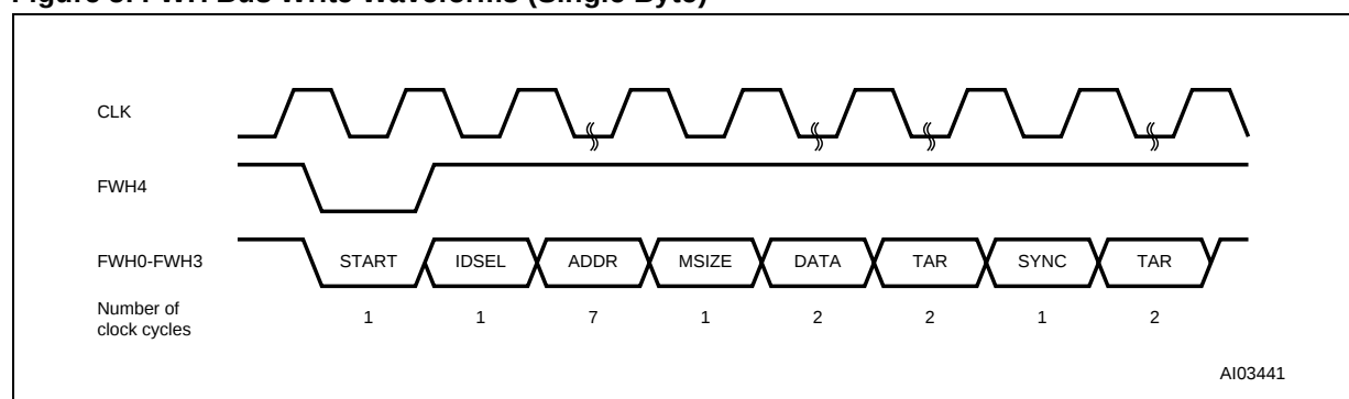
Figure 5. FWH Bus Write Waveforms (Single Byte)
