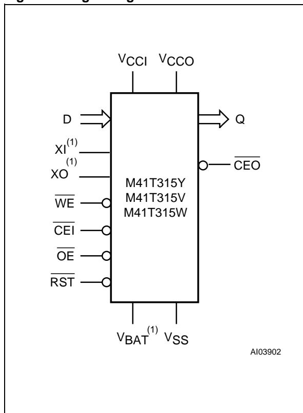
Figure 3. Logic Diagram
