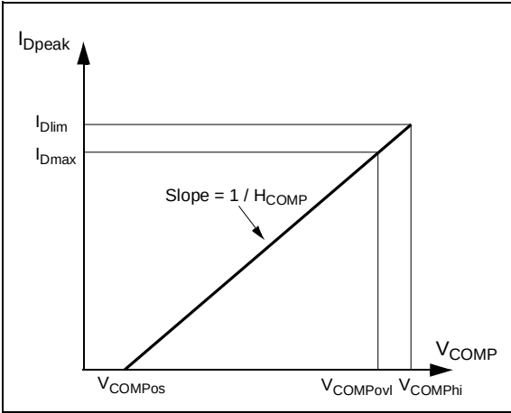
Figure 8: Comp Pin Gain and Offset
