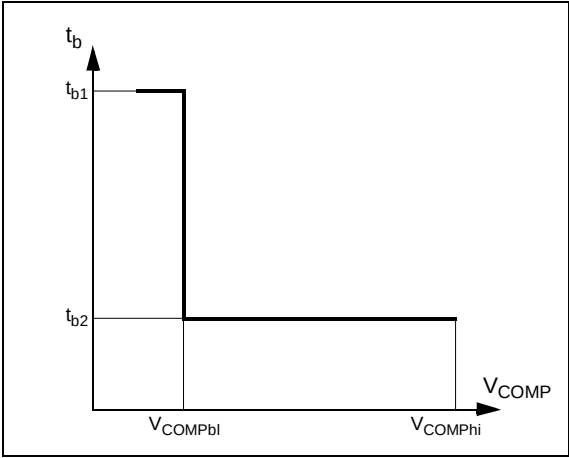
Figure 11: Blanking Time
