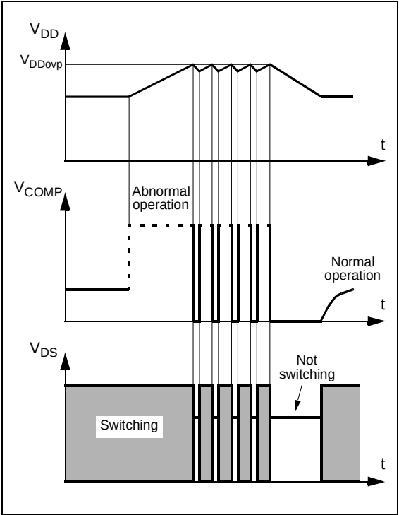
Figure 7: Overvoltage Event
