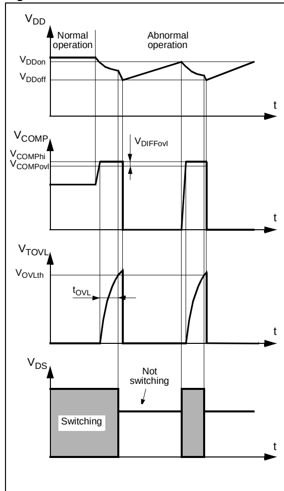
Figure 4: Overload event
