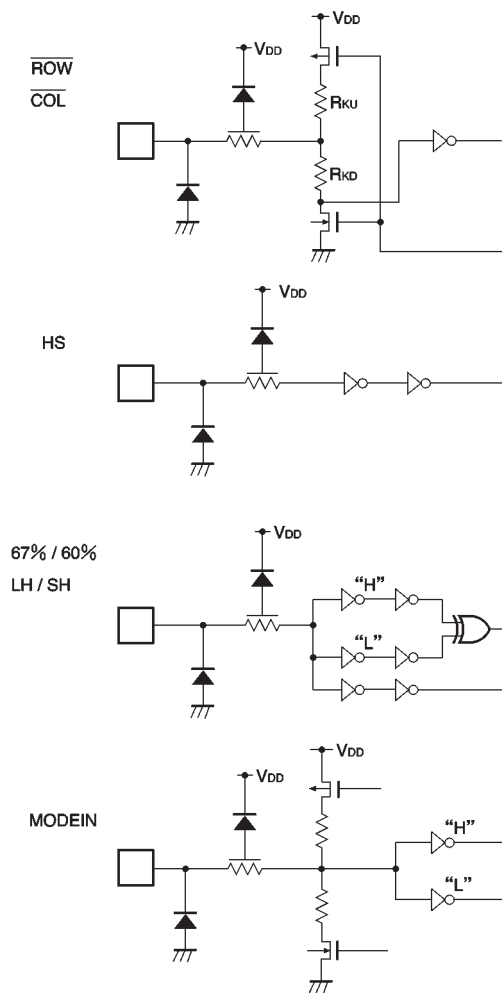
Fig. 12 Input interface circuit
