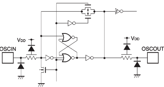
Fig. 13 Oscillation circuit
