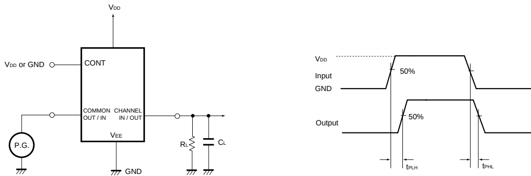
Fig. 4 Propagation delay time (Switch IN to OUT)
