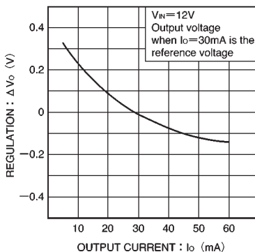
Fig. 3 Load regulation
