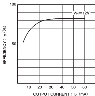
Fig. 2 Efficiency
