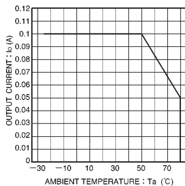
Fig.7 Derating curve
