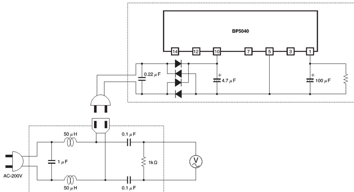
Fig.6 Test circuit
