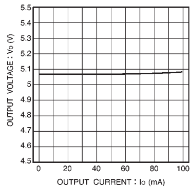
Fig.9 Output characteristic
