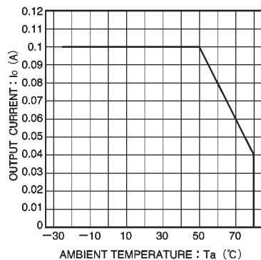
Fig.6 Derating curve
