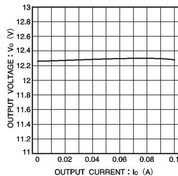
Fig.8 Output characteristic
