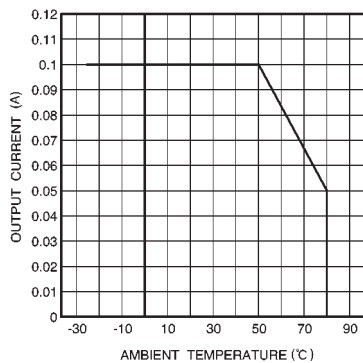
Fig.14 Derating curve
