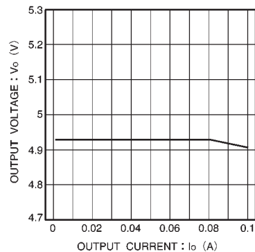
Fig.16 Output characteristic
