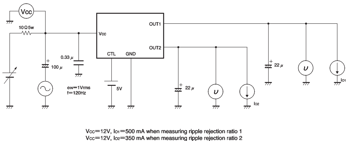
Fig.2 Circuit for measuring ripple rejection ratio
