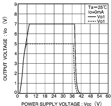
Fig.10 Output voltage characteristics (Typ.)
