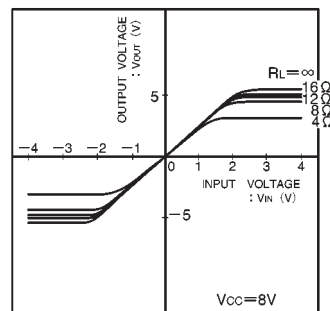
Fig. 11 Driver I / O characteristics (when power supply voltage power changes) (except channel 2)
