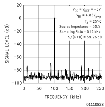
Spectral Response with 100 kHz Sine Wave Input
