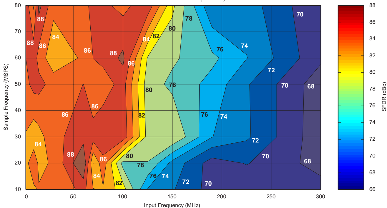
SPURIOUS-FREE DYNAMIC RANGE (SFDR) WITH DLL OFF
