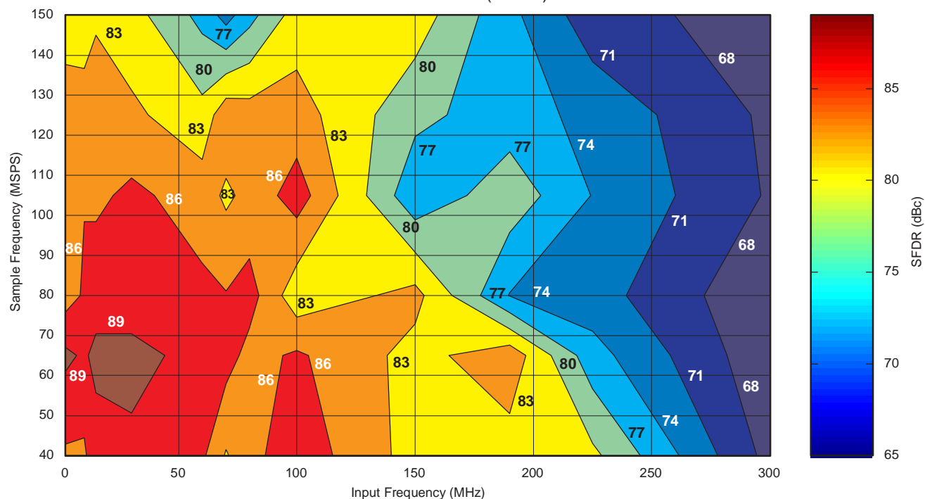
SPURIOUS-FREE DYNAMIC RANGE (SFDR) WITH DLL ON
