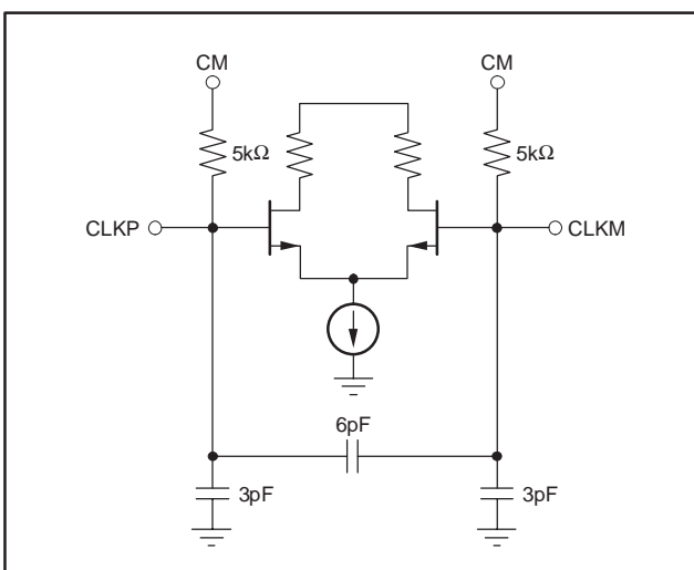
Figure 9. Clock Inputs
