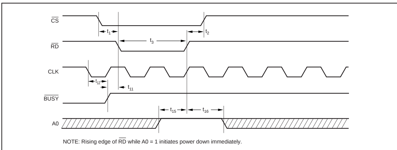
FIGURE 5. Entering Power-Down Using \overline{\text{RD}} and A0.
