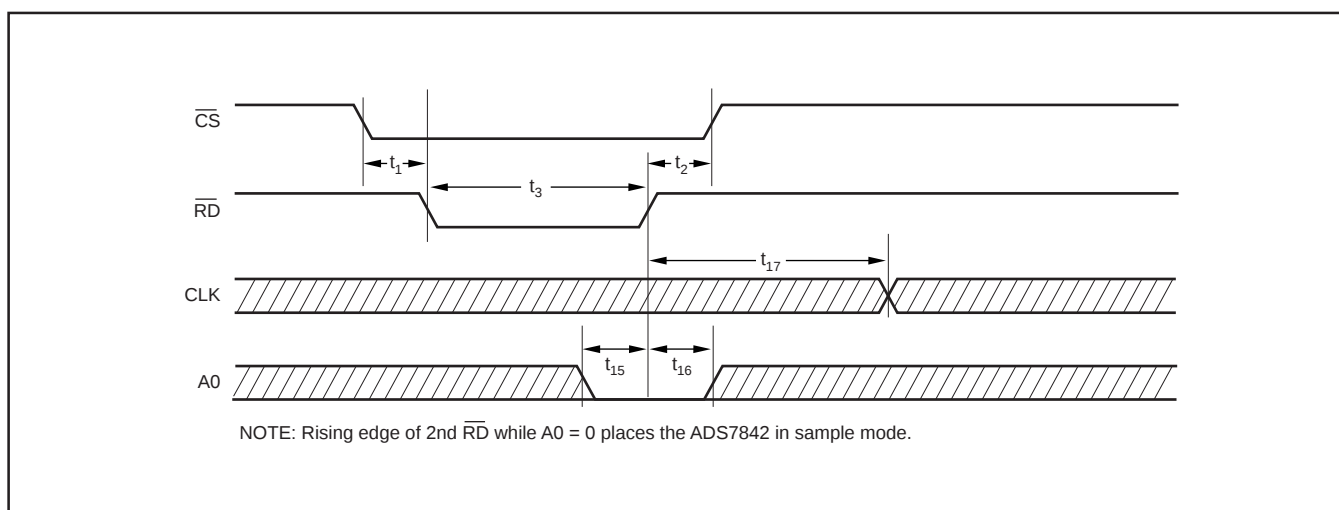
FIGURE 6. Initiating Wake-Up Using \overline{\text{RD}} and A0.
