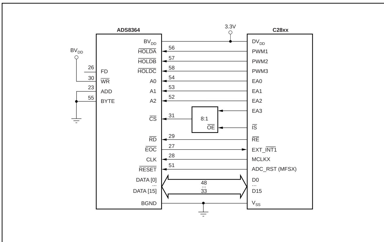
FIGURE 13. Typical F28xx Connection (Hardware Control).
