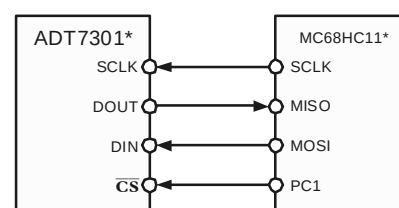
Figure 4. ADT7301 to MC68HC11 Interface
