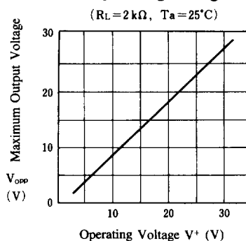
Maximum Output Voltage vs. Operating Voltage
